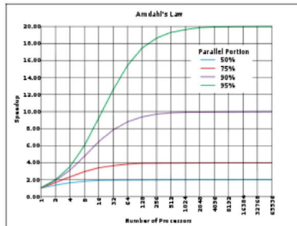
Figure 1. A graphical representation of Amdahl's law.
